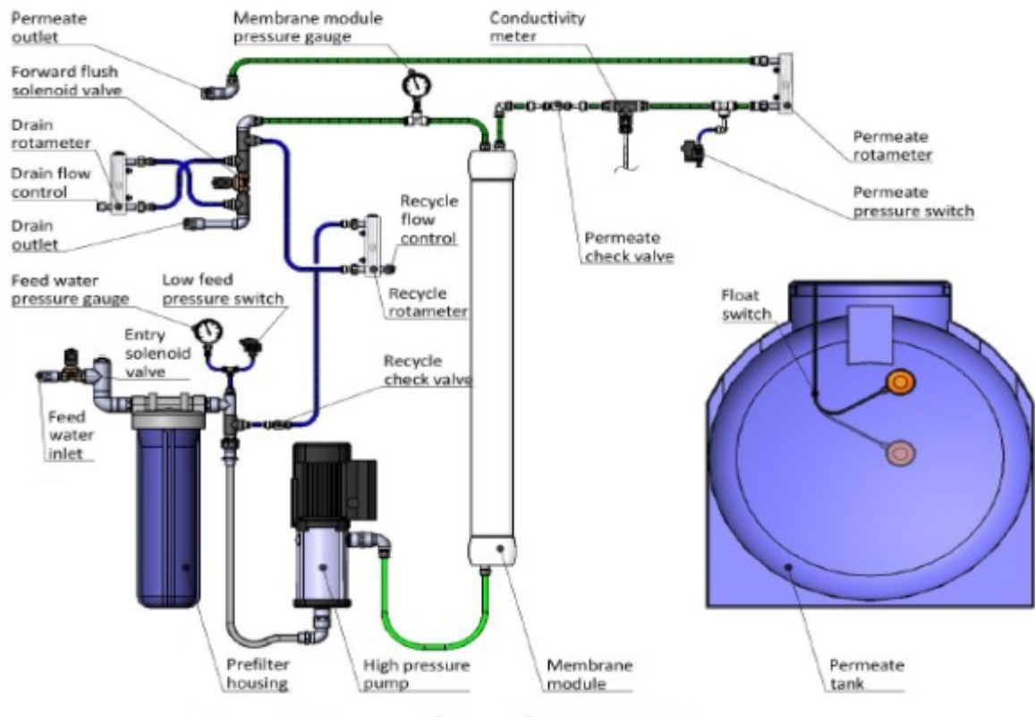
Figure 2. Layout of Ecosoft MO 6000
