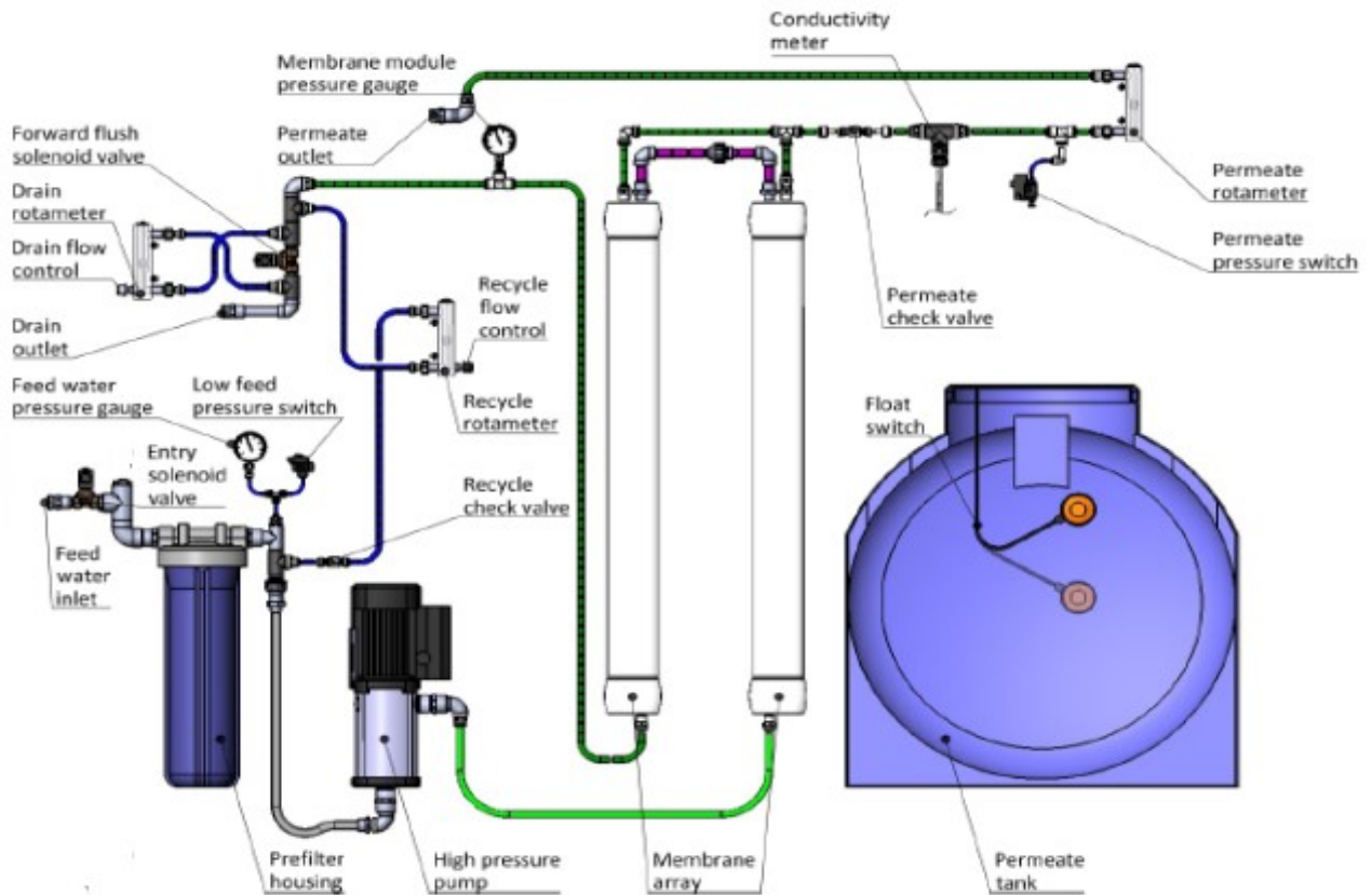
Figure 3. Layout of Ecosoft MO 12000
