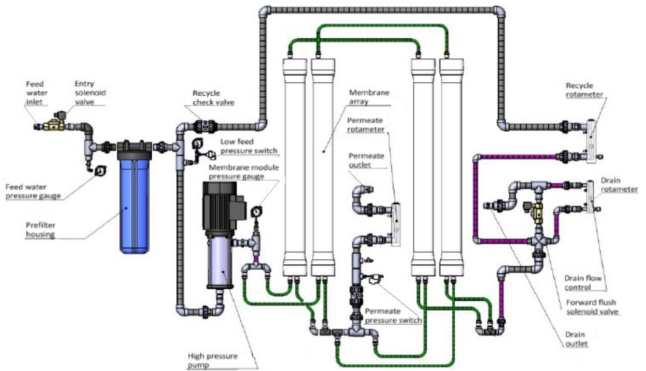
Figure 4. Layout of Ecosoft MO 24000
