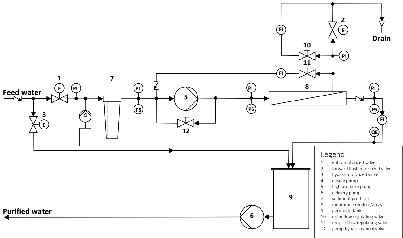
Figure 1. Reverse osmosis system with raw water blending
