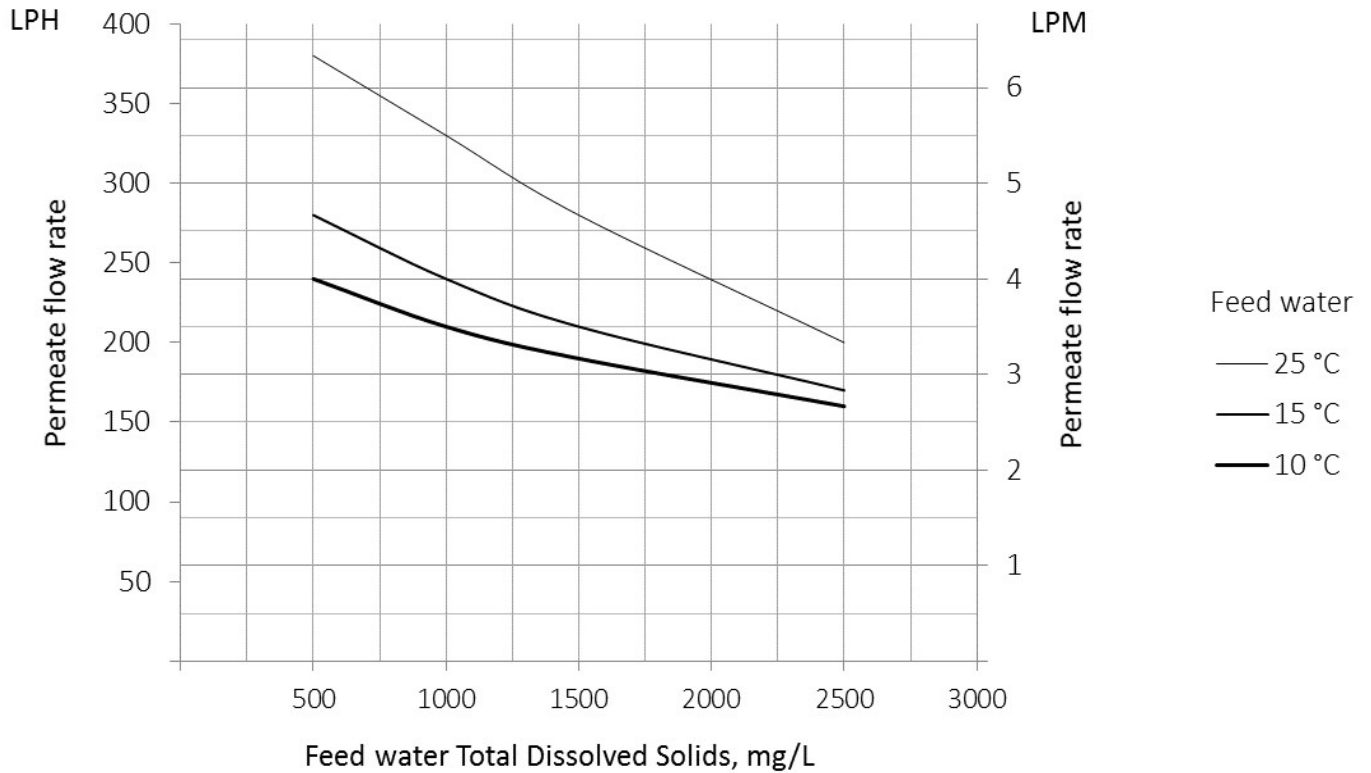
Figure 1. TDS/Flow rate curves for MO6000
