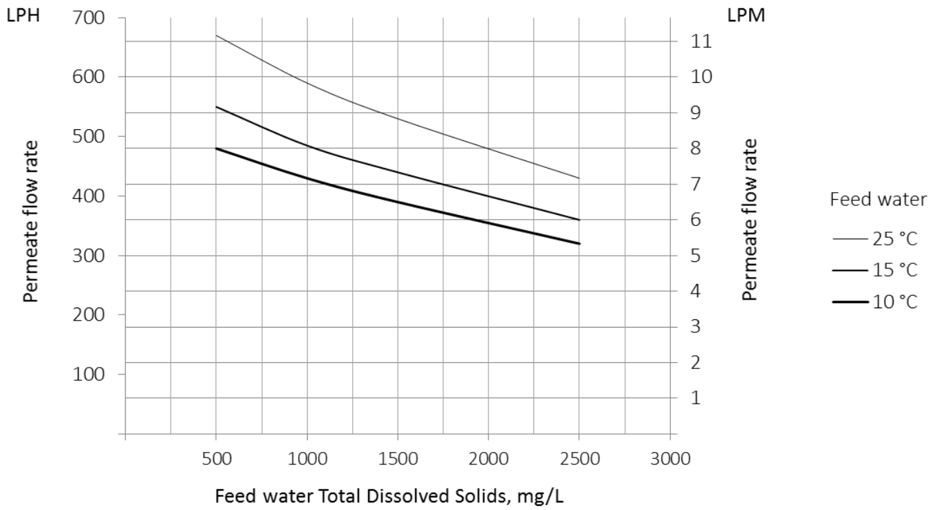
Figure 2. TDS/Flow rate curves for MO12000
