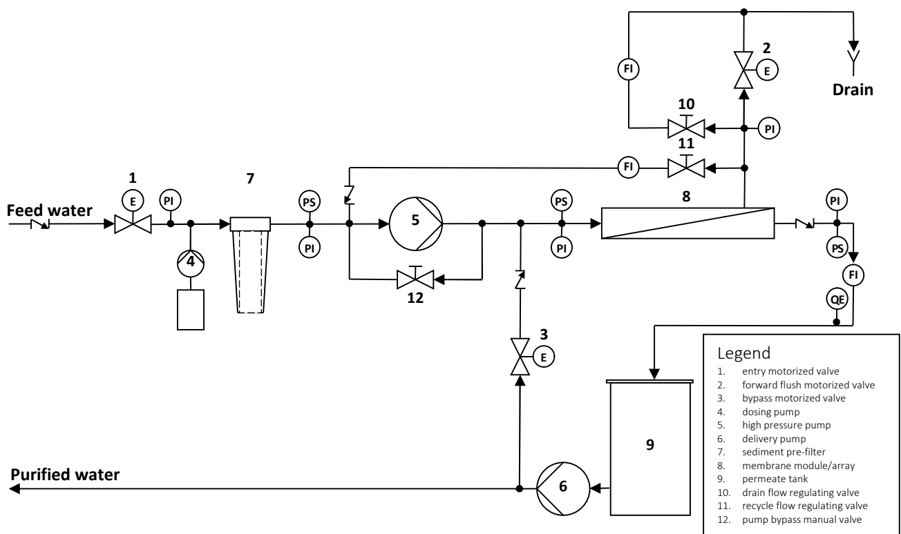
Figure 2. Reverse osmosis system with permeate rinsing
