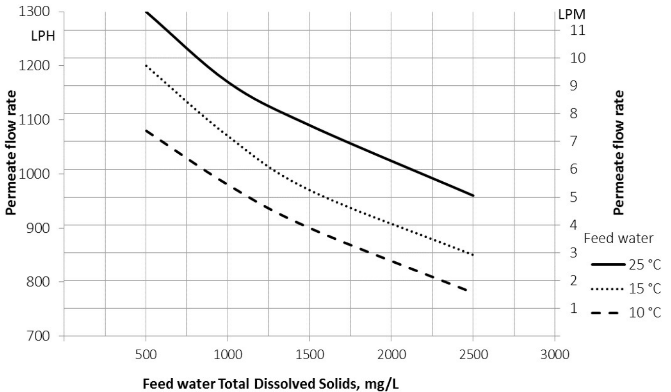
Figure 3. TDS/Flow rate curves for MO24000
